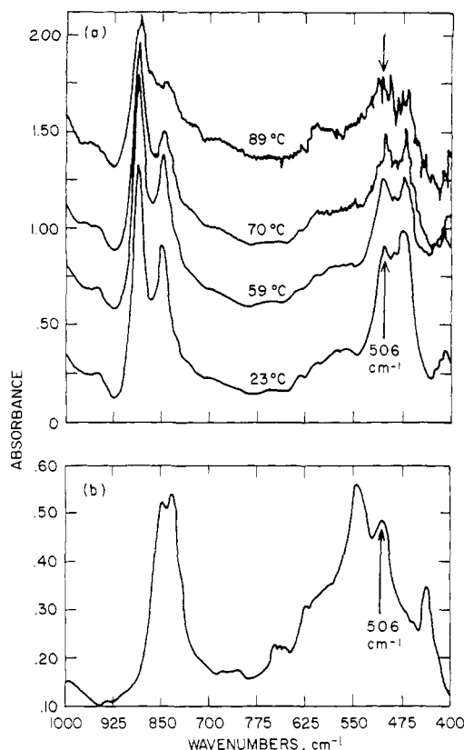
Figure 7. (a) Infrared spectra of copolymer samples at a series of temperatures. Spectra for elevated temperatures have been displaced vertically for clarity. (b) Infrared spectrum of poly-(trifluoroethylene) at room temperature.
