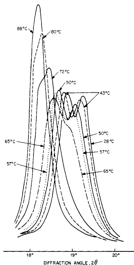
Figure 4. X-ray diffractometric scans from unoriented, unpoled copolymer films at various temperatures. The diffraction angles are those for Cu K\alpha radiation ( \lambda = 0.15418\text{ nm} ).
