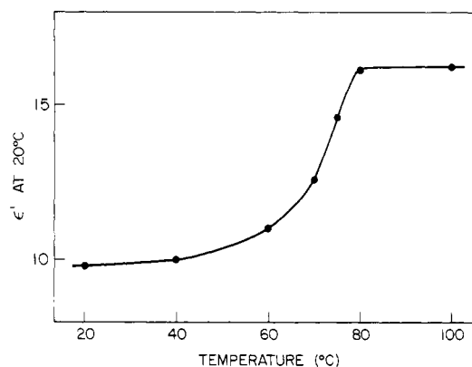
Figure 3. Change of \epsilon' of 20^\circ\text{C} as a result of heating of poled copolymer.
