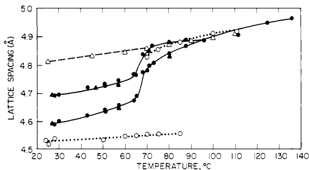
Figure 6. Variation of intermolecular spacing with temperature for various samples: (●) unoriented, unpoled copolymer; (○) unoriented, poled copolymer; (Δ) poly(trifluoroethylene). Data points indicated by solid triangles were obtained upon cooling from the highest temperature; all other data points were obtained upon heating.
