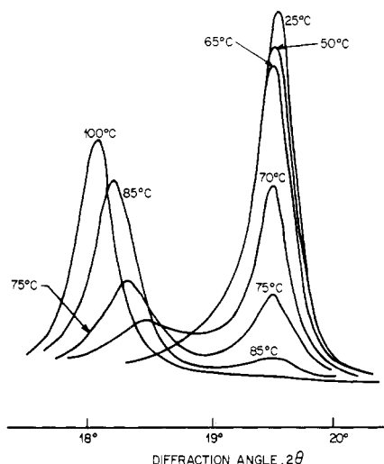
Figure 5. X-ray diffractometer scans from unoriented but poled copolymer films at various temperatures. The diffraction angles are those for Cu K \alpha radiation ( \lambda = 0.15418 nm).
