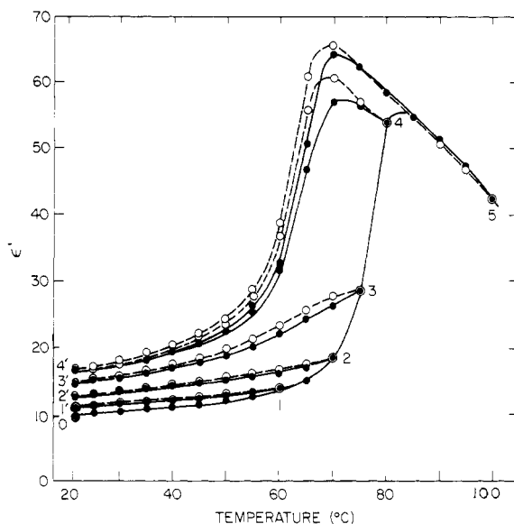
Figure 2. Change of \epsilon' of poled copolymer during heating and cooling cycles. Dashed line (open circles) indicates the cooling process, and solid line (filled circles) the heating process.
