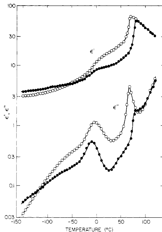
Figure 1. Temperature dependence of \epsilon' and \epsilon'' at 1 kHz for unpoled samples (open circles) and poled samples (filled circles).
